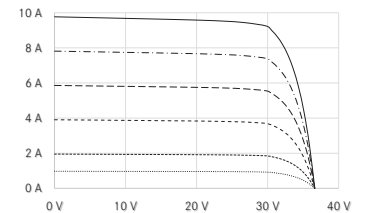
UI-diagramm e.g. LX-290M/156-60+
